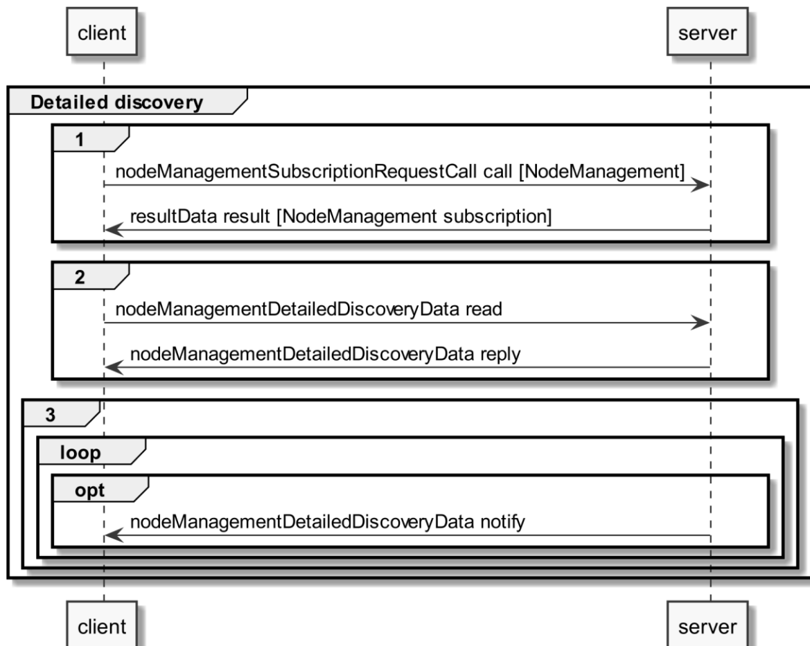
1424 Figure 9: Pre-Scenario communication - Detailed discovery sequence diagram
