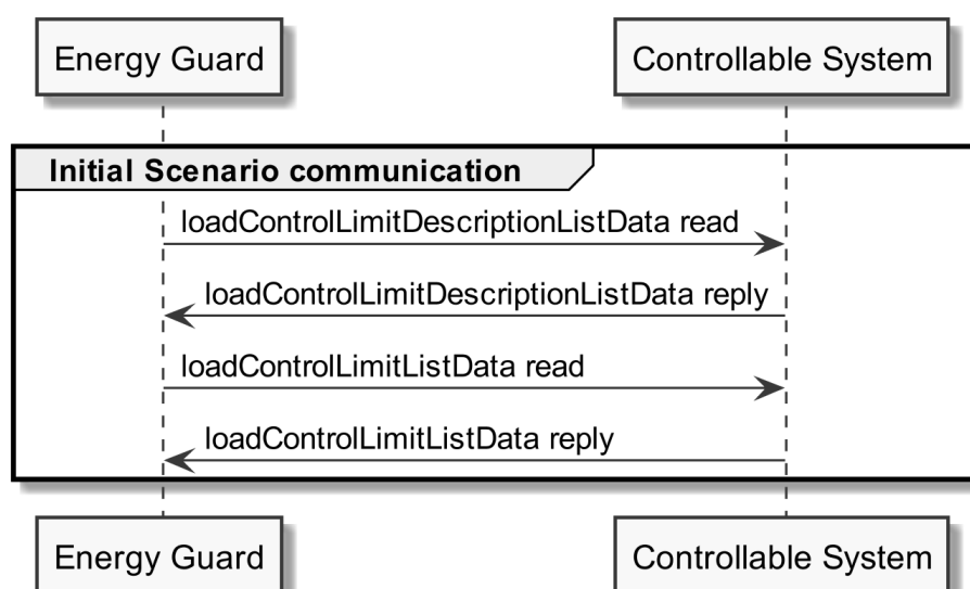
Figure 12: Scenario 1 - Initial Scenario communication sequence diagram
