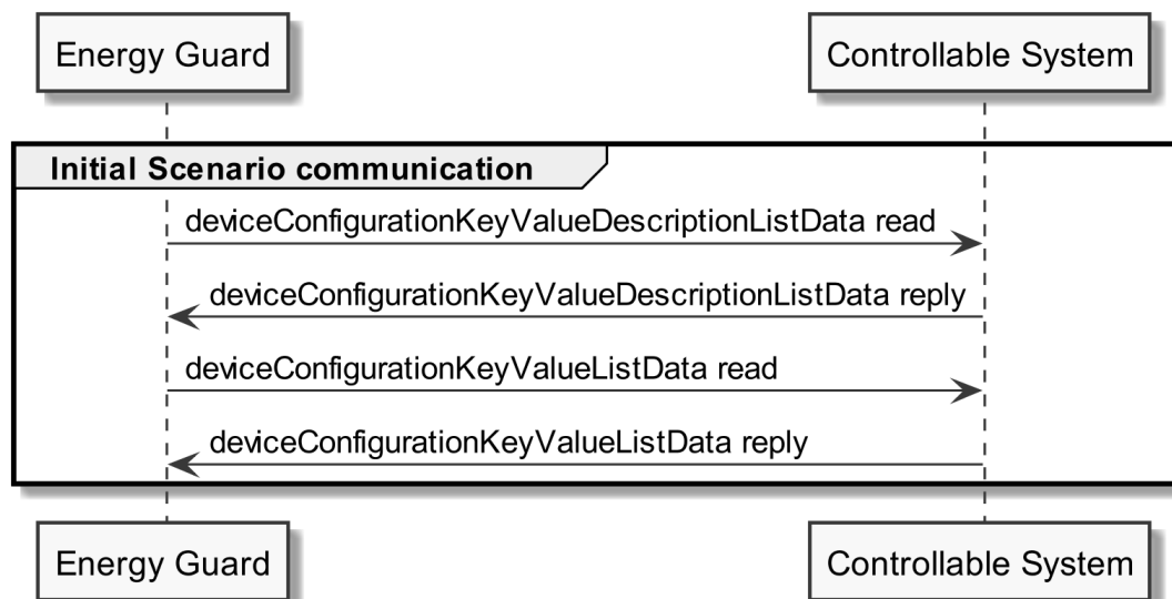
Figure 14: Scenario 2 - Initial Scenario communication sequence diagram
