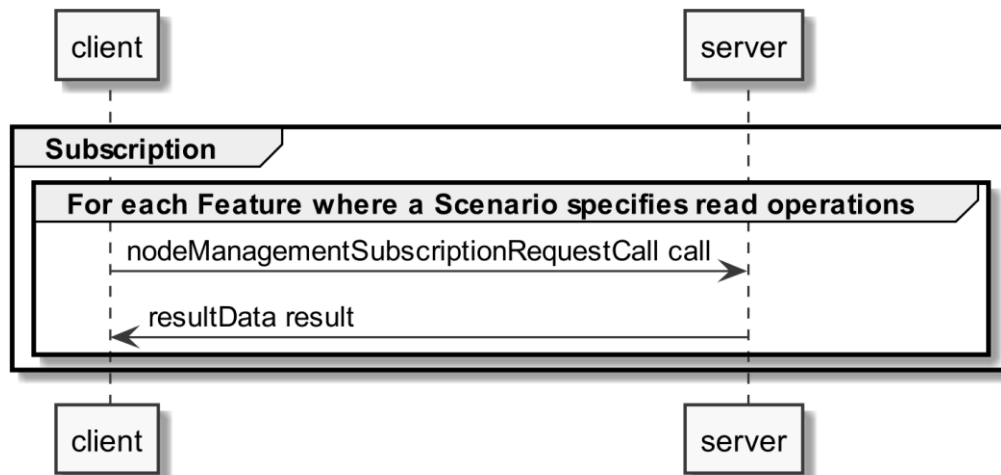
Figure 11: Pre-Scenario communication - Subscription sequence diagram
