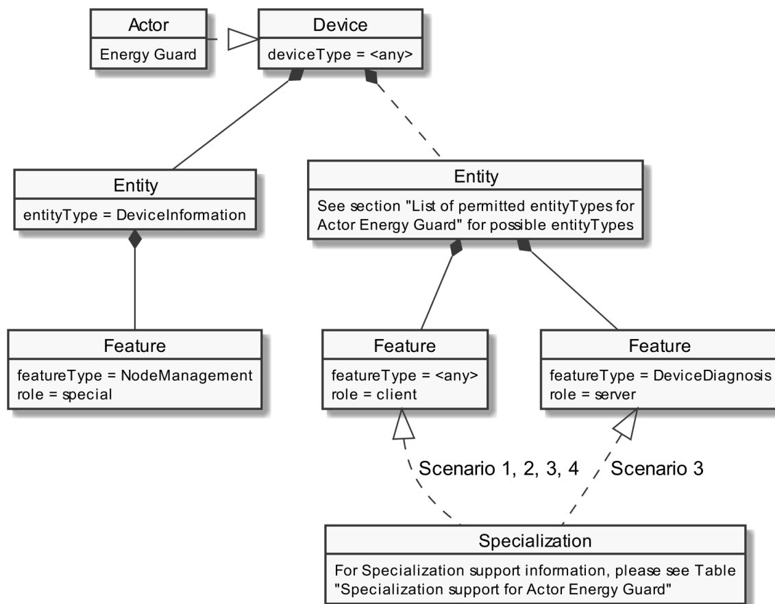
1185 Figure 7: Actor "Energy Guard" overview
