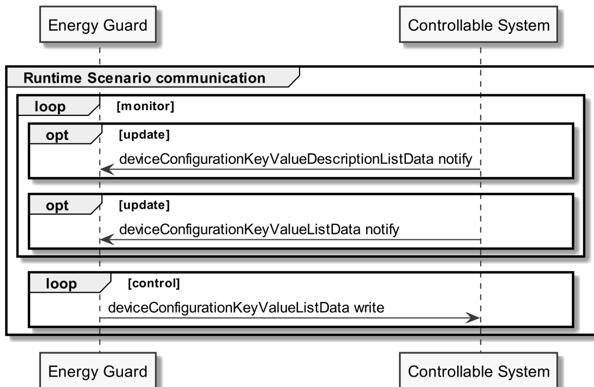
Figure 15: Scenario 2 - Runtime Scenario communication sequence diagram
