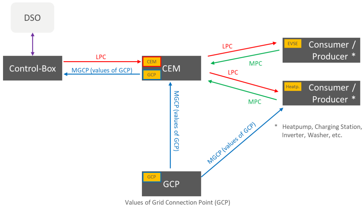
Figure 4: Example for cascading constellations of this Use Case, combined with the Use Cases MPC and MGCP
